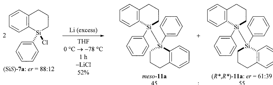
Scheme 5. Reductive metallation of (SiS)-7a accompanied by the formation of disilanes 11
