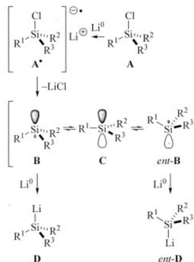
Scheme 2. Vertex inversion of silyl radicals ( R^1 \neq R^2 \neq R^3 )
