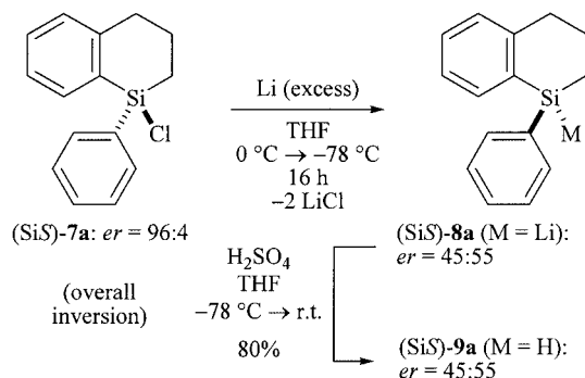
Scheme 3. Reductive metallation of (SiS)- 7a
