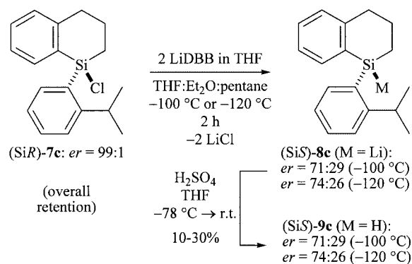
Scheme 8. Reductive metallation of (SiR)-7c
