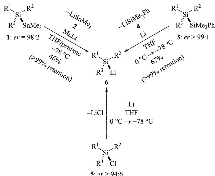
Scheme 1. Strategies for the enantioselective preparation of asymmetrically substituted silyl anions ( R^1 \neq R^2 \neq R^3 )
