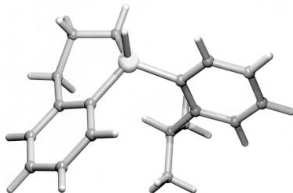
Figure 2. Molecular structure of (SiS)-9c
