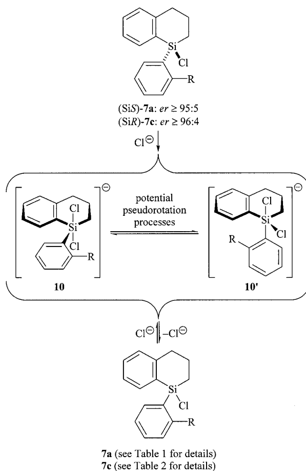
Scheme 4. Plausible mechanisms for the chloride-induced racemisation of chiral silyl chlorides 7
