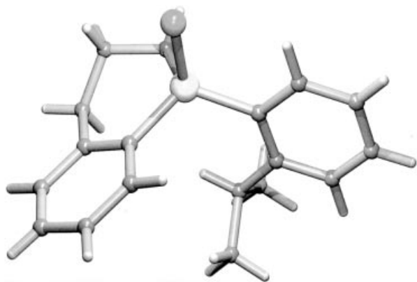
Figure 3. Molecular structure of (SiR)-7c
