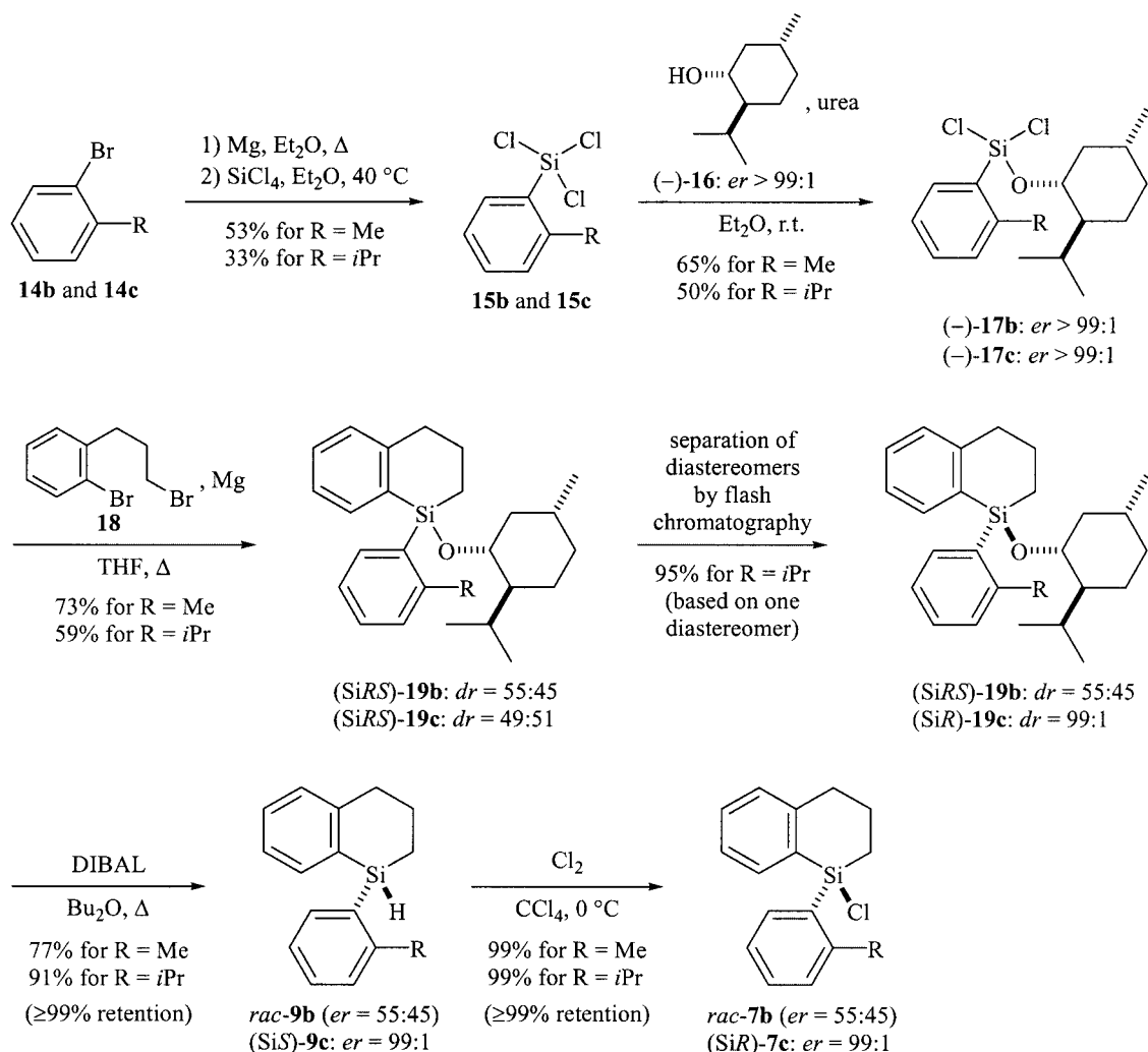
Scheme 7. Preparation of the sterically hindered silyl chlorides rac -7b and (SiR)-7c
