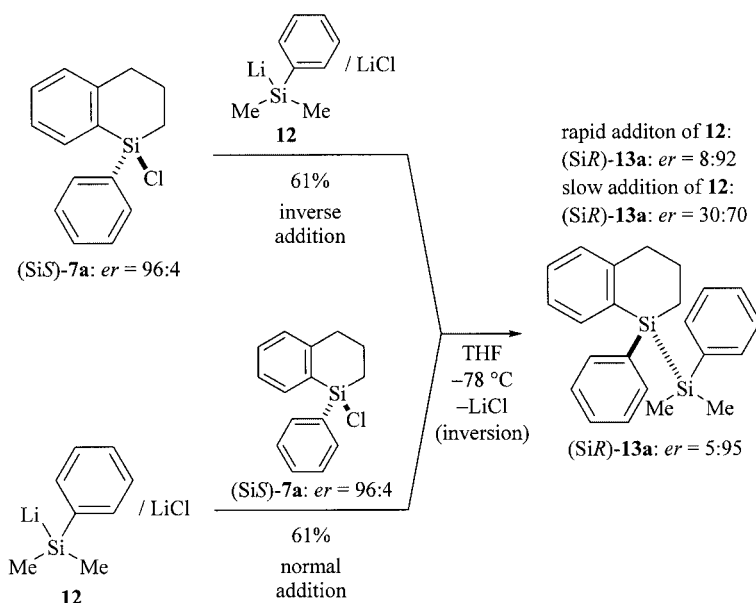
Scheme 6. Nucleophilic displacement at (SiS)- 7a using the achiral silyl anion 12
