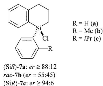
Figure 1. 1-Aryl-1-chloro-1,2,3,4-tetrahydro-1-silanaphthalenes 7
